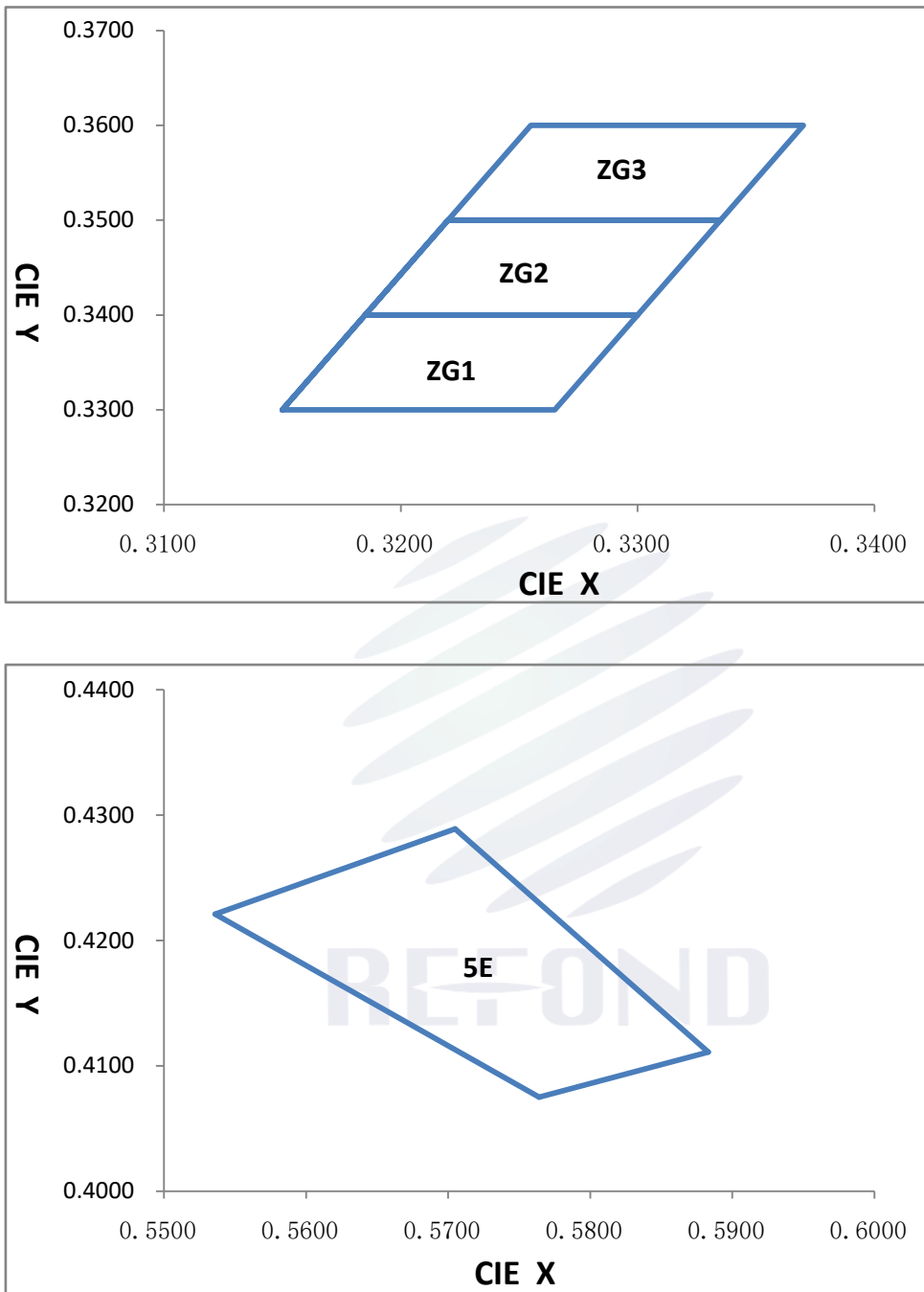
Fig 1-6 The C.I.E Chromaticity Diagram CIE色度图
