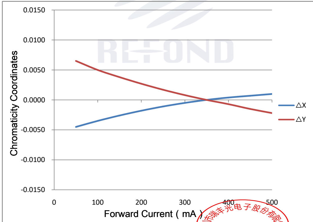
Fig. 1-13 Chromaticity Coordinate Shift Vs Forward Current (Amber) 色坐标与电流特性曲线(琥珀光)
