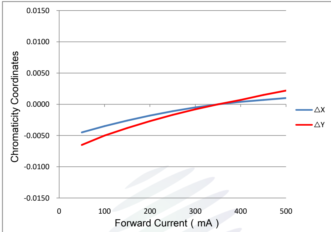
Fig. 1-13 Chromaticity Coordinate Shift Vs Forward Current (White) 色坐标与电流特性曲线(白光)
