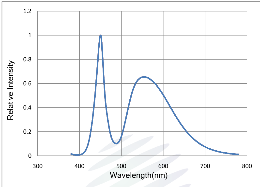
Fig. 1-14 Spectrum Distribution(White)光谱分布特性曲线 (白光)
