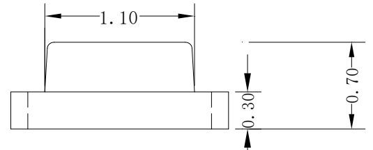
Fig.1-2 Side view 侧面视图
