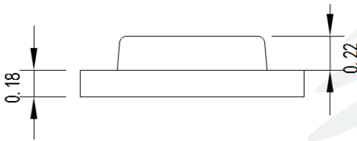
Fig.1-3 Side view 侧面视图
