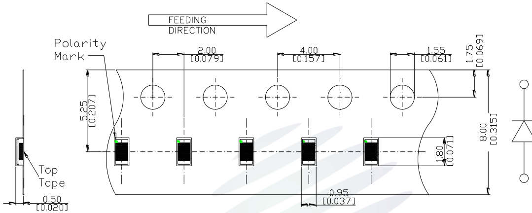
Fig.2-1 Carrier Tape Dimension 载带尺寸
