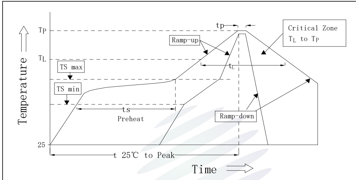
Fig.3-1 SMT Reflow Soldering Instructions SMT 回流焊说明
