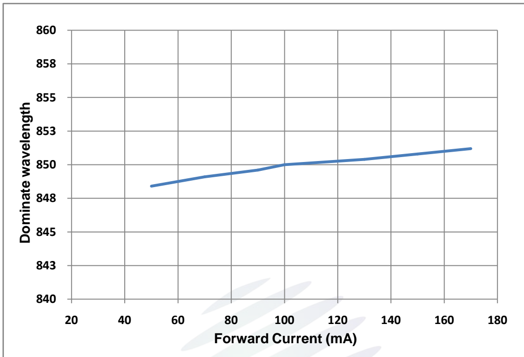
Fig. 1-13 Forward current vs. Dominate wavelength (Ts=25°C)正向电流与主导波长特性曲线(Ts=25°C)
