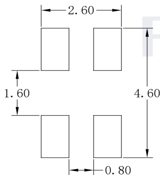
Fig. 1-5 Soldering Patterns 推荐焊盘
