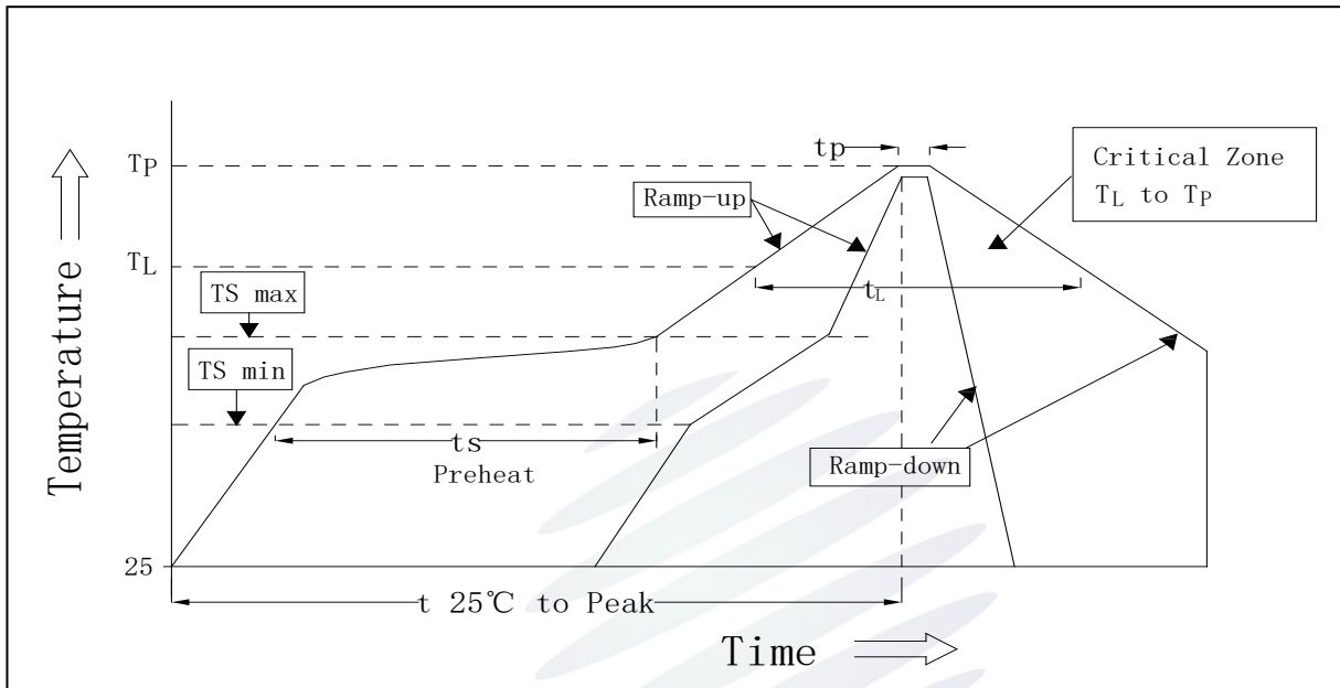
Fig.3-1 SMT Reflow Soldering Instructions SMT 回流焊说明
