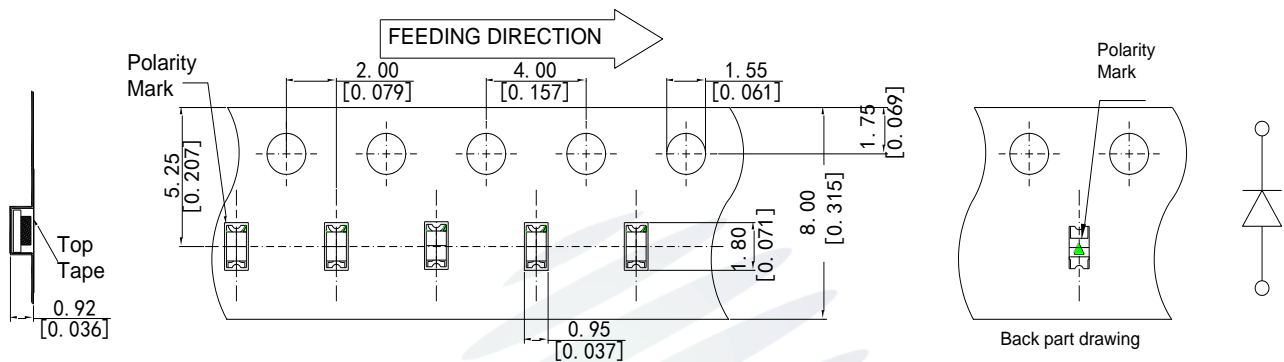
Fig.2-1 Carrier Tape Dimension 载带尺寸
