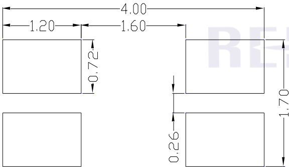
Fig.1-5 Soldering patterns 推荐焊盘
