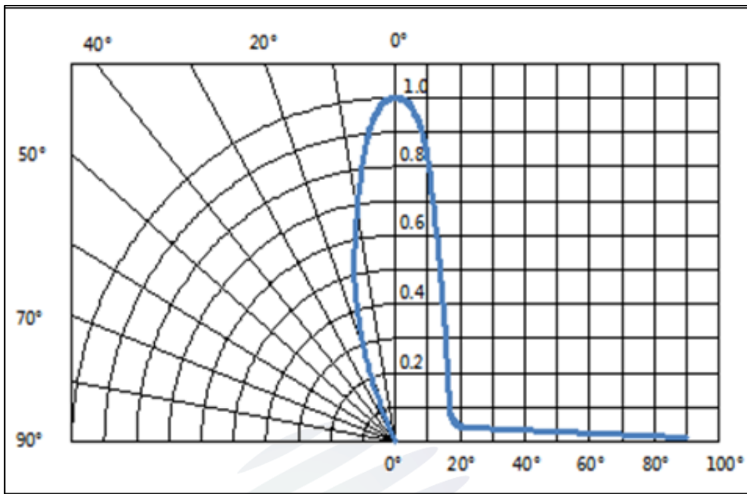
Fig.1-12 Diagram characteristics of radiation 辐射特性曲线
